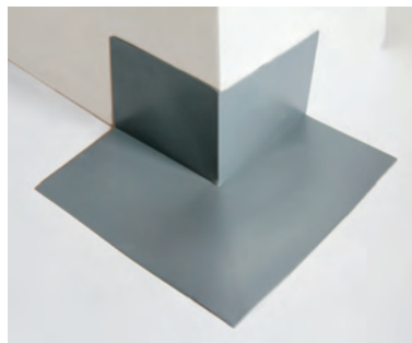
Sealing membrane for outside corners 100 x 100 mm Art. No. 71
